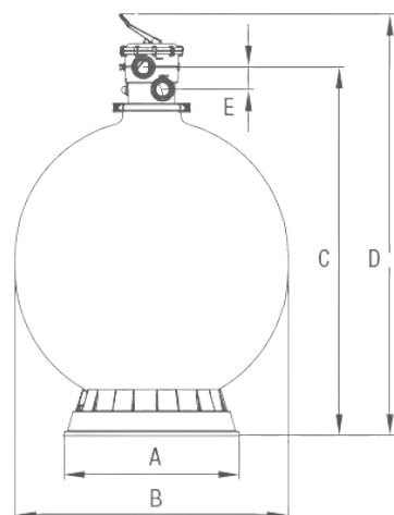
DIMENSIONS (MM/IN)
