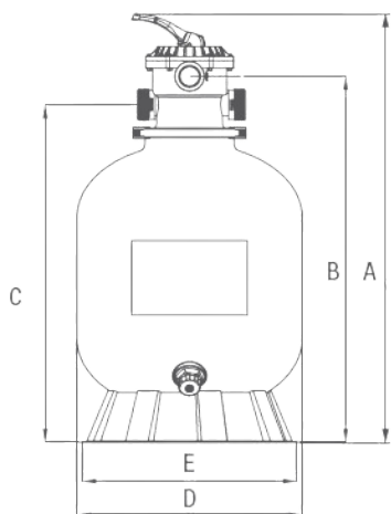
DIMENSIONS (MM/IN)
