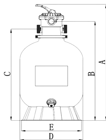
DIMENSIONS (MM/IN)
